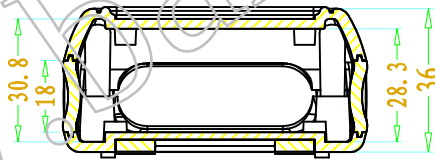
SEC B-B
