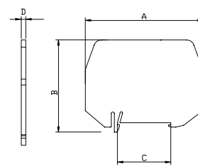
High Type Separation Plate Code: 1060527
