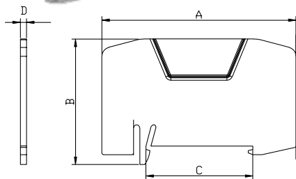
OPK Series Separation Plate New Code: 1060053 Old Code: 0592
