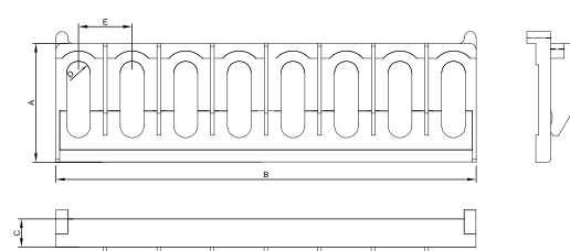
Upper Bridge for Test Sockets, 8 Poles New Code: 1060077 Old Code: 1302
