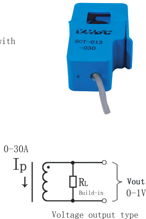
Schematic Diagram
