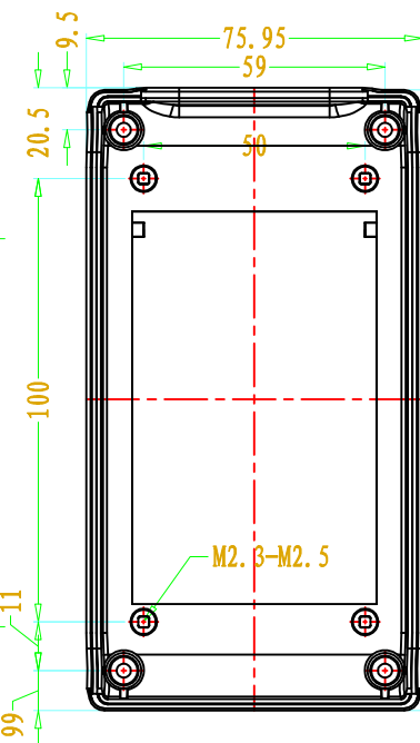
SEC B-B
